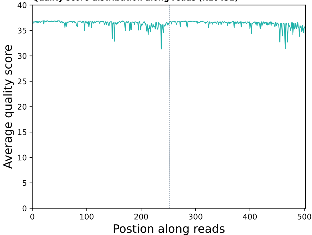
Quality score distribution along reads (R10431)
